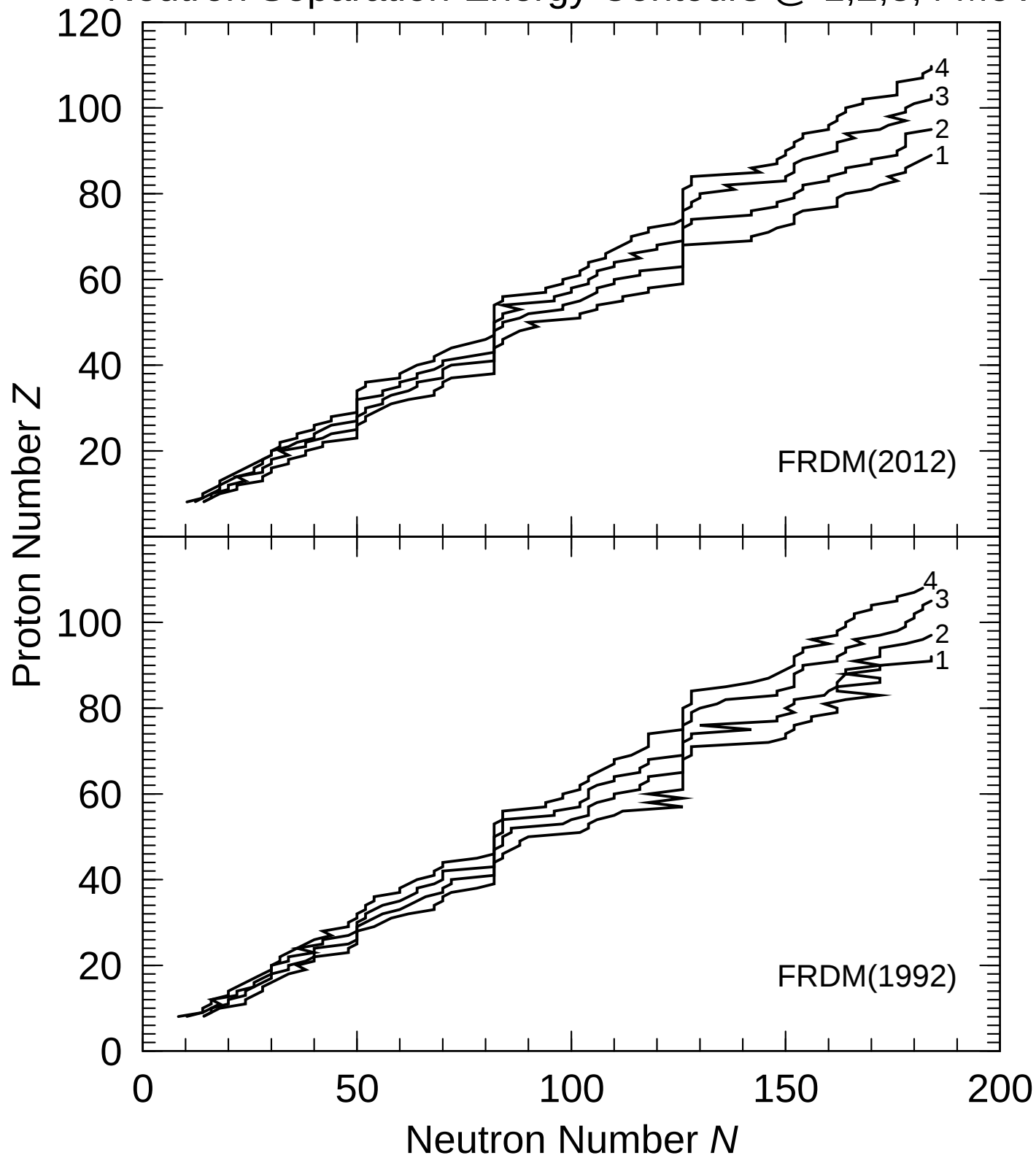
Neutron Separation-Energy Contours @ 1,2,3,4 MeV
