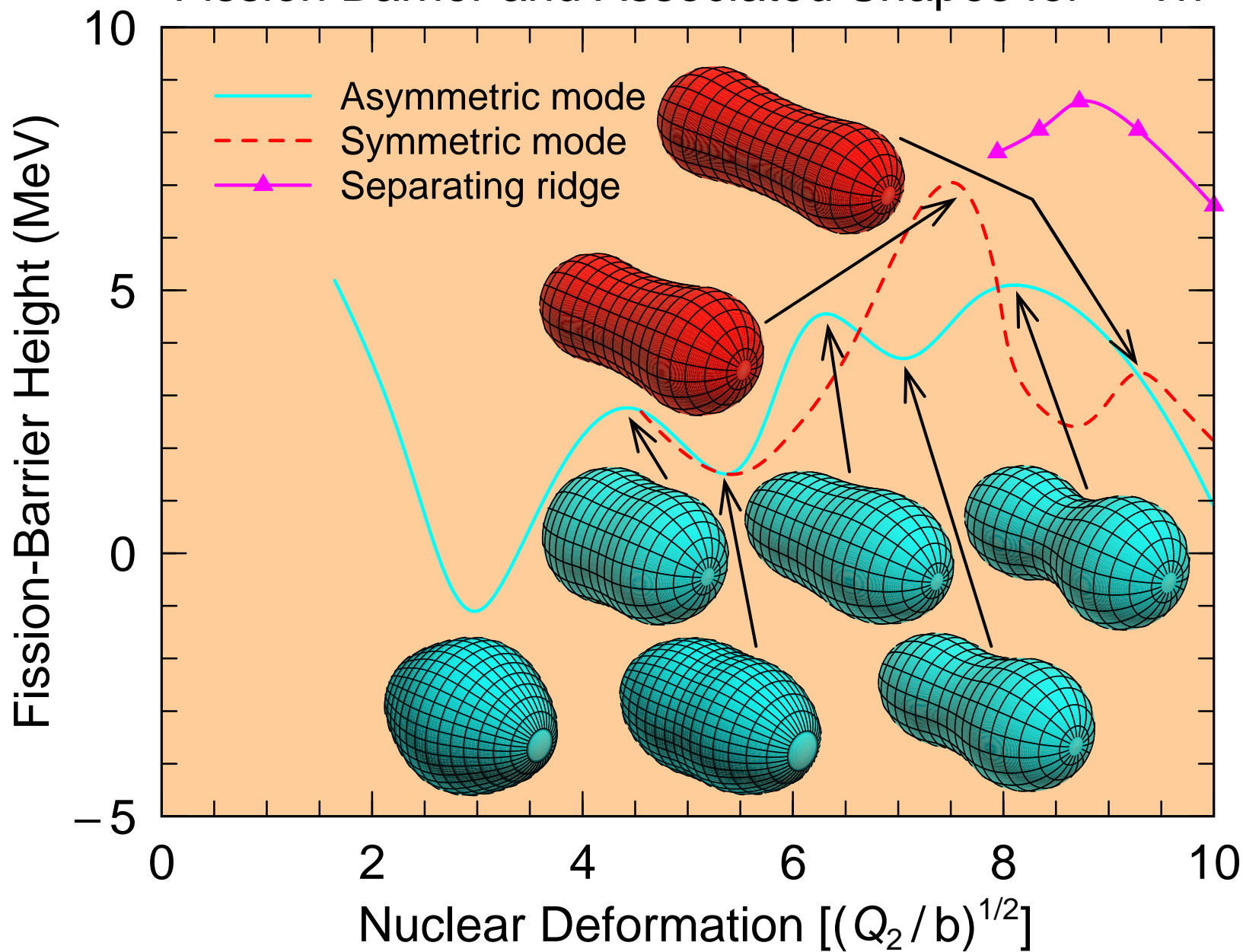
Fission Barrier and Associated Shapes for ^{232}\text{Th}
